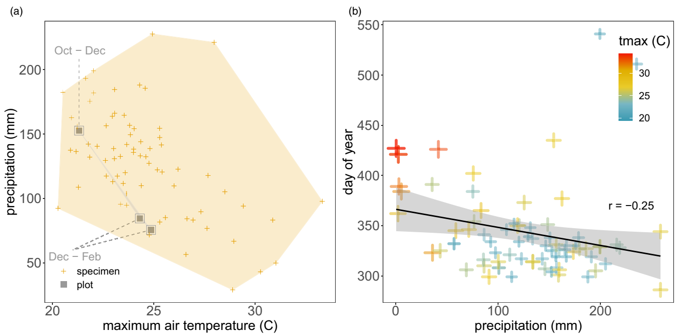
FIGURE 6 Amphiphium crucigerum phenology and its relationship with climate. (a) Flowering phenology field observations (grey squares) versus herbarium specimens (yellow crosses) are depicted in climate space. Maximum air temperature and precipitation represent monthly averages of the year/location of collection/observation, respectively. Crosses represent specimens and grey squares represent surveyed plots. Grey text insets indicate the flowering periods of this species as surveyed in each plot. (b) The relationship between day of year flowering and mean September–October precipitation inferred from herbarium specimens. Both field observation data and specimen data indicated that A. crucigerum flowering begins in October and persists into the following year.
