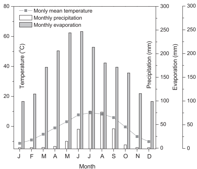
Fig. 2. Monthly mean air temperature, monthly total precipitation, and monthly evaporation from 1957 to 2013 in Baingoin (4700 m a.s.l.), about 100 km north-west of the Nam Co Lake.
