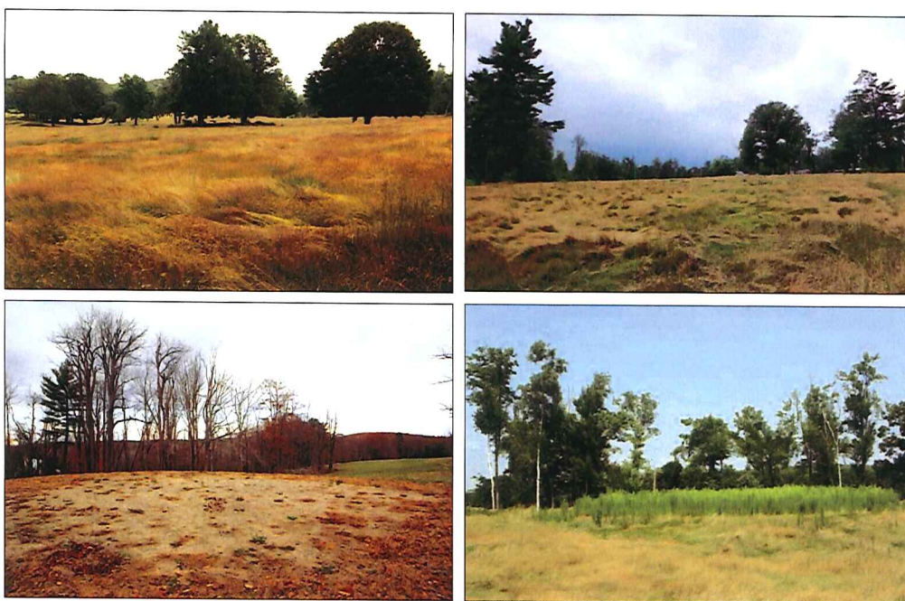
Figure 6. Former fairways (top) and putting greens (bottom) at PCC. In 2014, most plots on fairways were dominated by Agrostis capillaris and/or Poa pratensis . Estimates of the cover of individual grass species were difficult because grasses were ‘matted down’ (upper right) when sampling occurred in mid- to late-summer. Grasses (e.g., A. capillaris ) that formerly dominated most putting greens died in 2013 or 2014, leaving extensive areas of exposed ‘duff’ (light gray areas in lower left photo). In 2014, putting greens supported dense stands of tall Erigeron canadensis (bottom right, bright green) above the exposed ‘duff’ layer.
